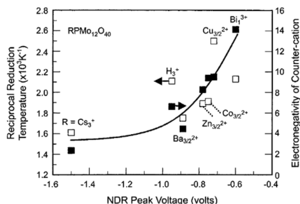
Fig. 3. Correlation between NDR peak voltage of cation-exchanged \text{RPMo}_{12}\text{O}_{40} ( \text{R}=\text{H}_3^+ , \text{Cs}_3^+ , \text{Ba}_{3/2}^+ , \text{Zn}_{3/2}^{2+} , \text{Co}_{3/2}^{2+} , \text{Cu}_{3/2}^{2+} , \text{Bi}_1^{3+} ) HPAs and Tanaka electronegativity of the counter-cation (filled squares), and between NDR peak voltage and reciprocal reduction temperature of the HPAs (open squares).
