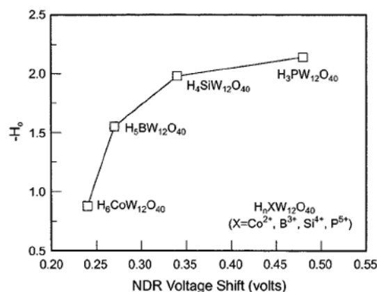
Fig. 6. Correlation between acid strengths of \text{H}_n\text{XW}_{12}\text{O}_{40} (X= \text{P}^{5+} , \text{Si}^{4+} , \text{B}^{3+} , \text{Co}^{2+} ) HPAs and their NDR voltage changes after pyridine exposure.
